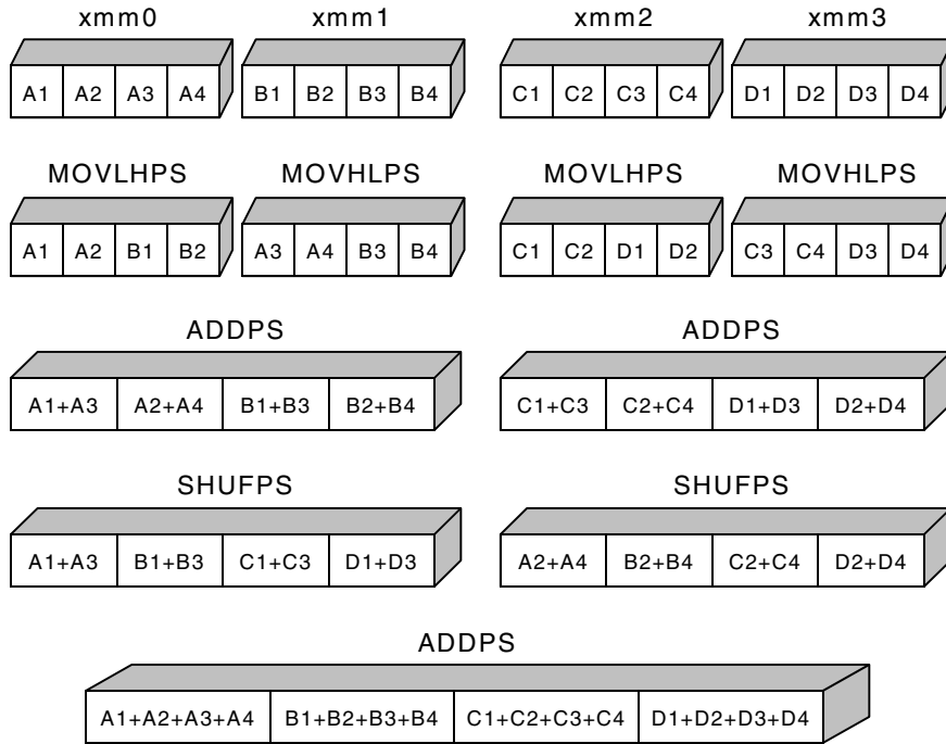
Figure 5-2 Horizontal Add Using movhpls/movhlps
